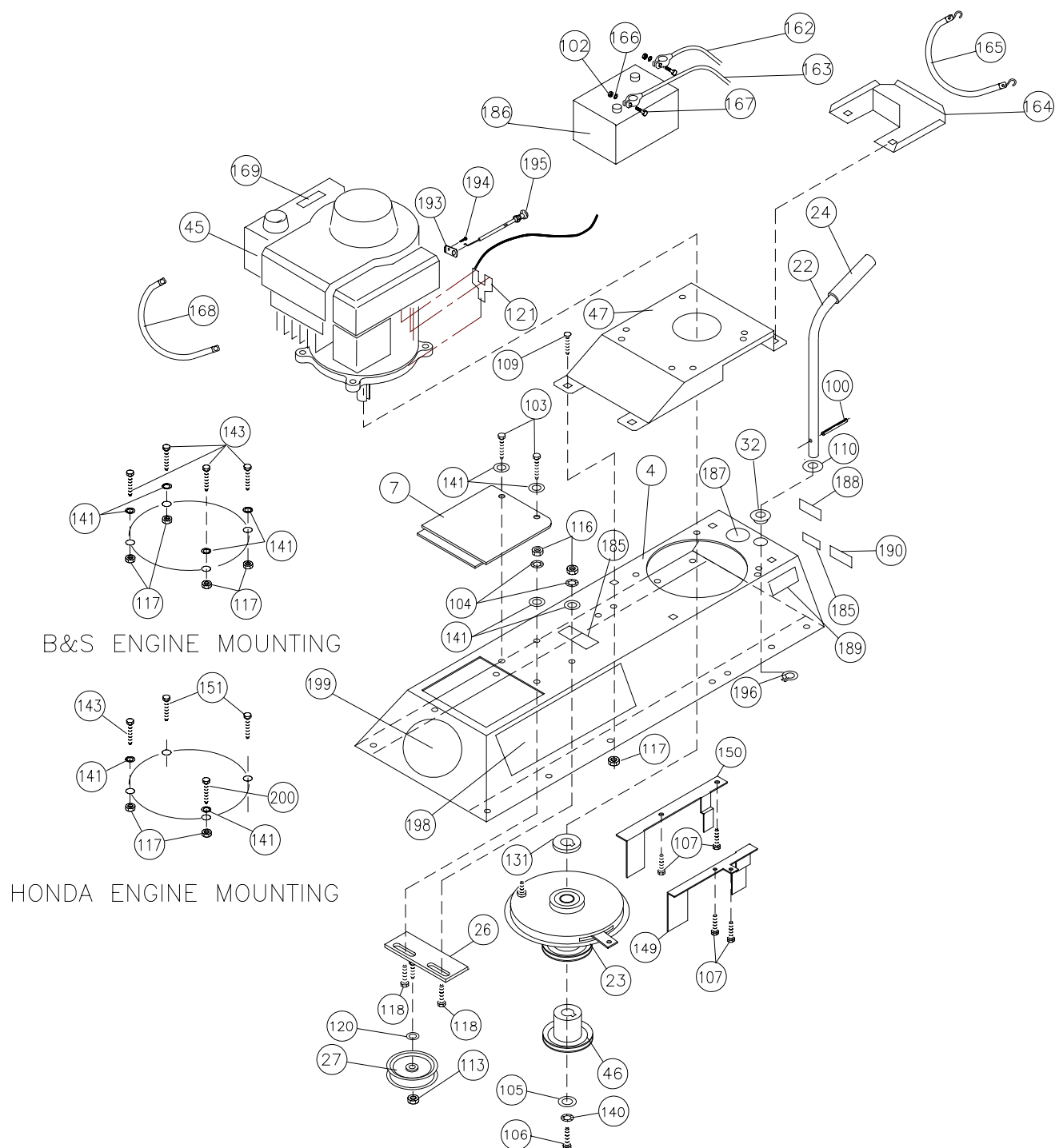
Engine and Engine Base Assembly Figure 6
