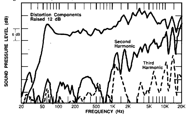
Figure 6. Harmonic Distortion at 0.1 Rated Power (25 watts, See Note 7)
