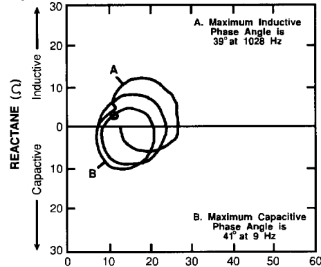
Figure 4. Complex Impedance
