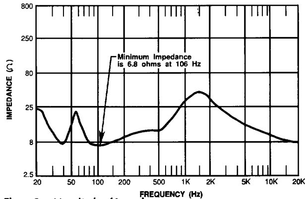
Figure 3. Magnitude of Impedance
