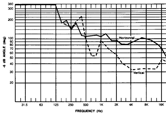
Figure 8. Coverage Angle
