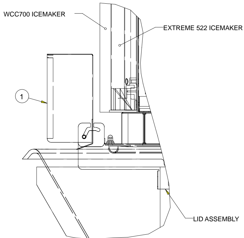
FIGURE 3b. OPEN POSITION SCALE 0.250
