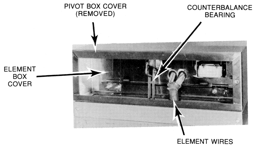
TOP VIEW FROM REAR
