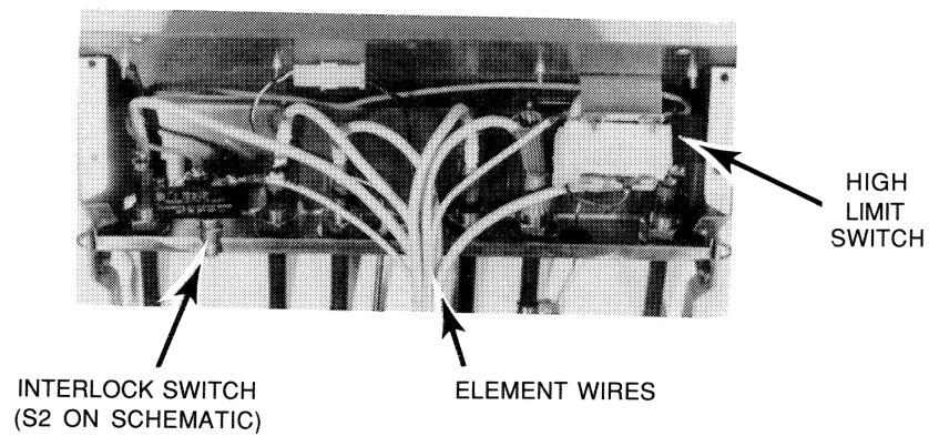
ELEMENT PIVOT BOX ASSEMBLY
