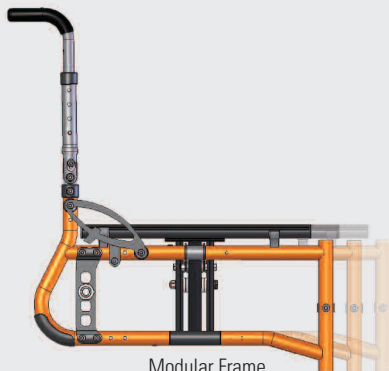
Modular Frame
