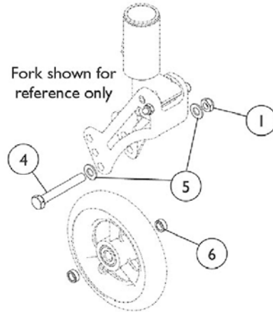
Suspension Forks
