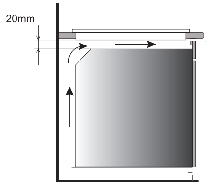
Installing hob in kitchen cabinet worktop above oven.
