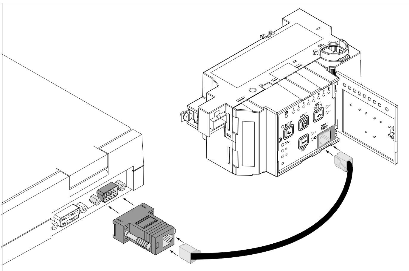
Figure 1: Controller front panel serial cable connection
