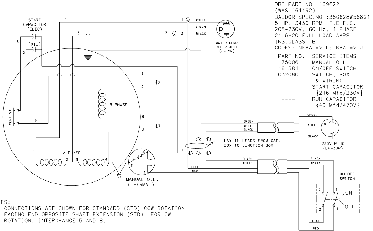
FIGURE 9 – Wiring Diagram – 51E (5 HP, 208-230 Volts, 60 Hertz, 1 Phase Electric Motor) [Note: Same Electrical Schematic For P/N's 177014 & 169622 (Shown)] (P/N 177014 is P/N 169622 with 1/2" Cut From Motor Shaft)
