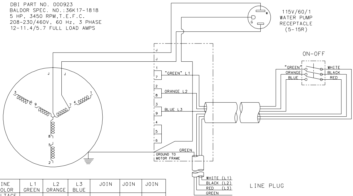
FIGURE 10 – Wiring Diagram – 53E (5 HP, 208-230 / 460 Volts, 60 Hertz, 3 Phase Electric Motor)
