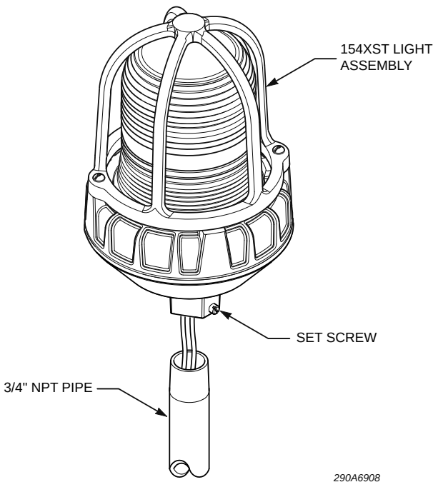
Figure 1 Pipe-mounted beacon
