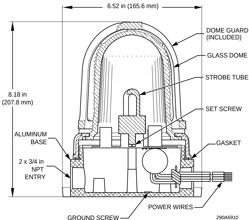
Figure 3 Cross section of lamp
