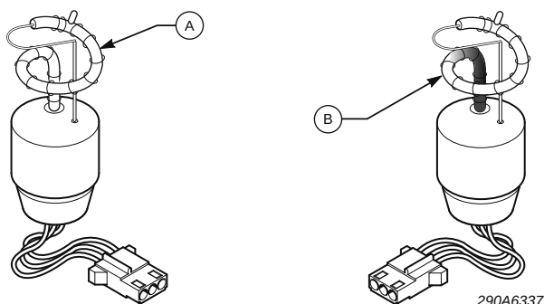
Figure 4 Normal (A) and darkened (B) flash tube
