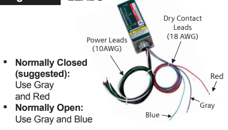
Figure 5 LEADS
