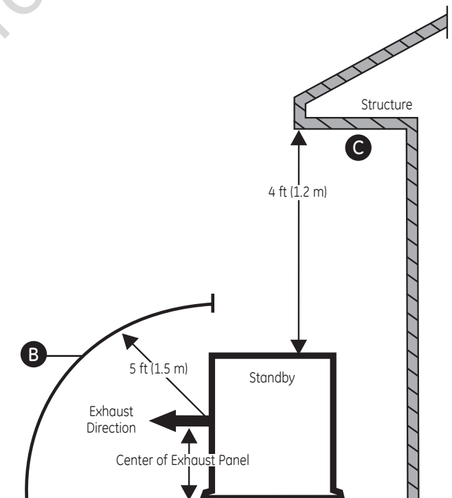
Vertical Clearances
