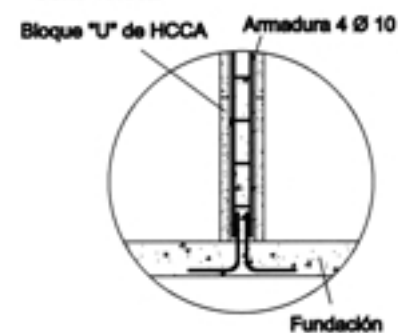
Corte vertical
