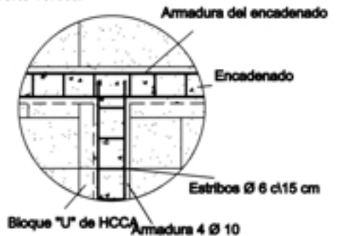
Corte vertical
