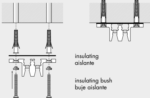
men sole multiple mounting montaje múltiple men sole
