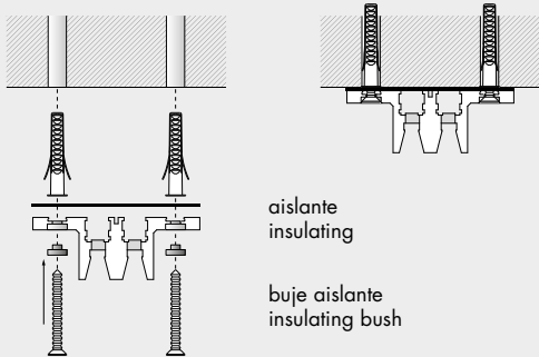
montaje múltiple men sole men sole multiple mounting
