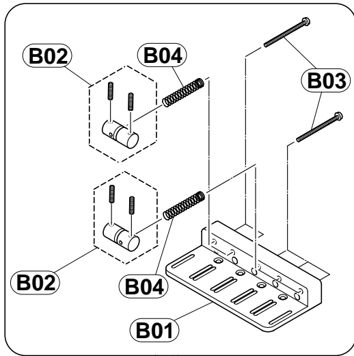
E11 Bridge Assembly BPX-5D ; GOLD (QC425400)
