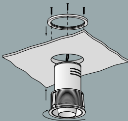
example of assembly displei recessed adjustable with ring nut for fastening from behind ejemplo de montaje displei empotrada orientable abrazadera panel plata
