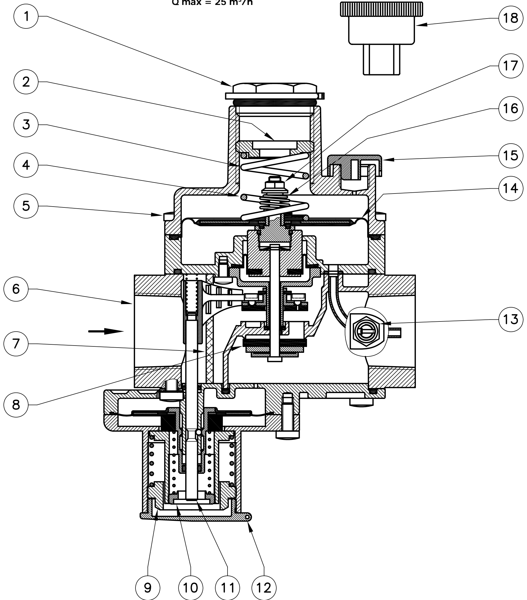
fig. 1: FRG/2MBC Q max = 25 m 3 /h
