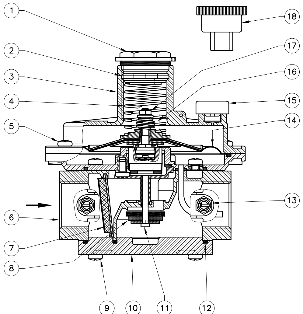
fig. 4: FRG/2MCS - RG/2MCS Q max = 100 m 3 /h
