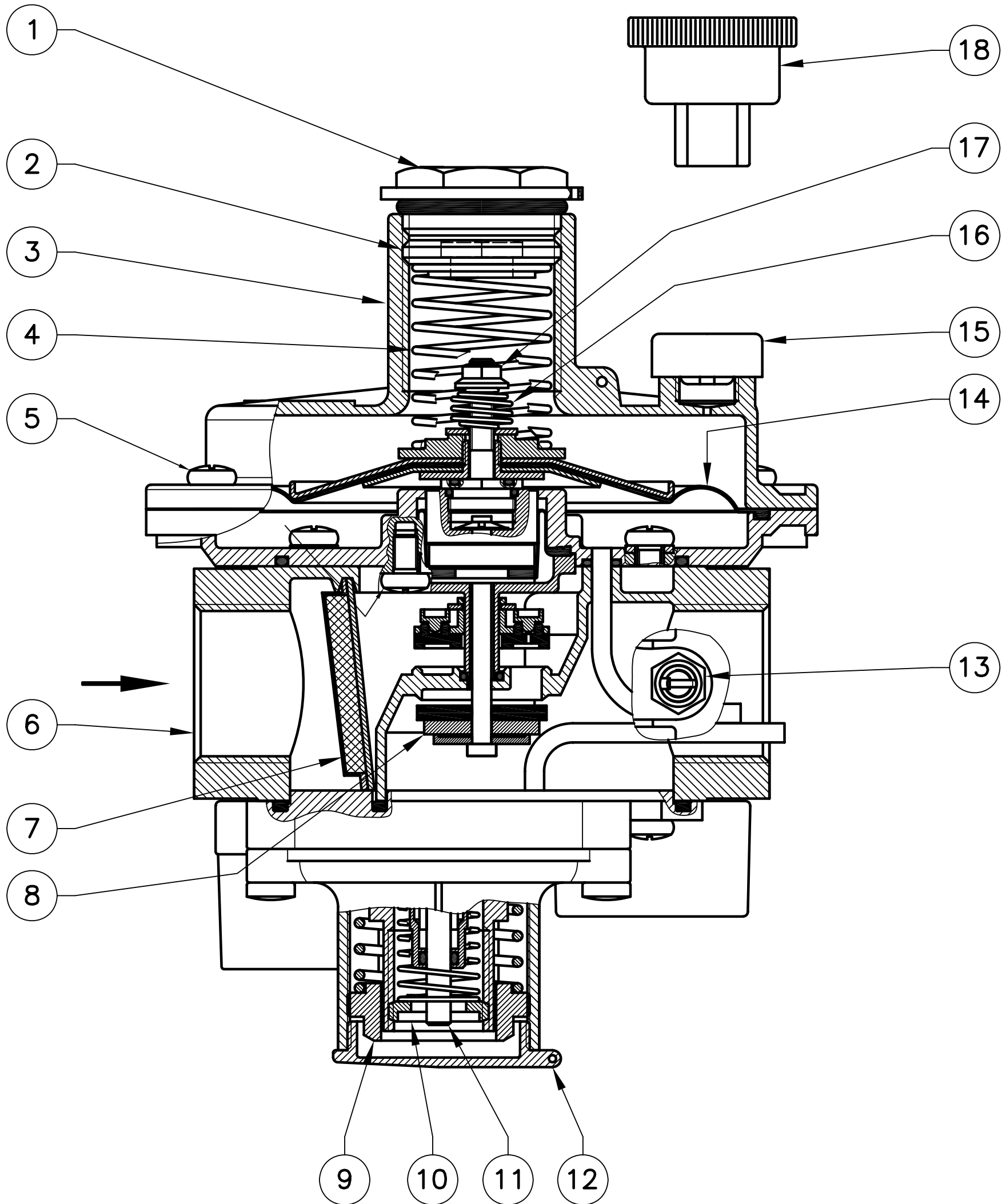
fig. 2: FRG/2MB Q max = 100 m 3 /h
