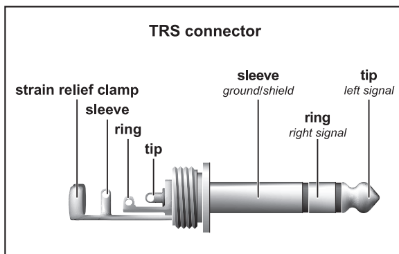
Fig. 5.2: 1/4" TRS stereo connector
