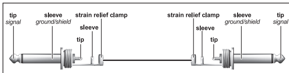
Fig. 5.1: Unbalanced instrument cable with 1/4" TS connector
