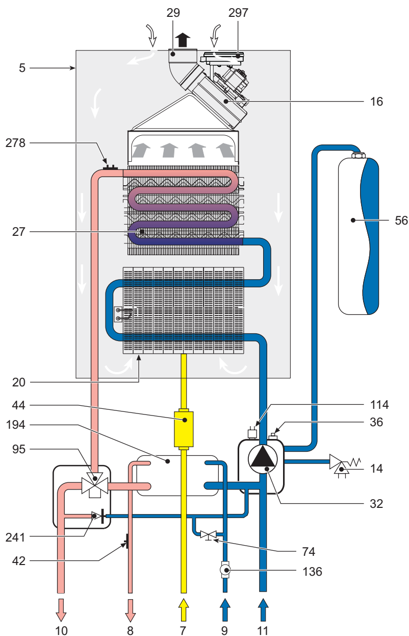
fig. 27 - Plumbing circuit
