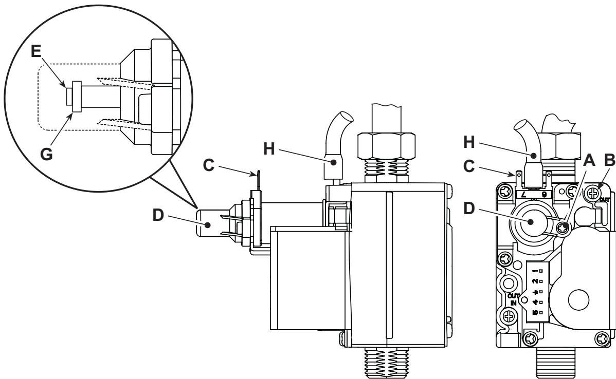
fig. 22 - Gas valve
