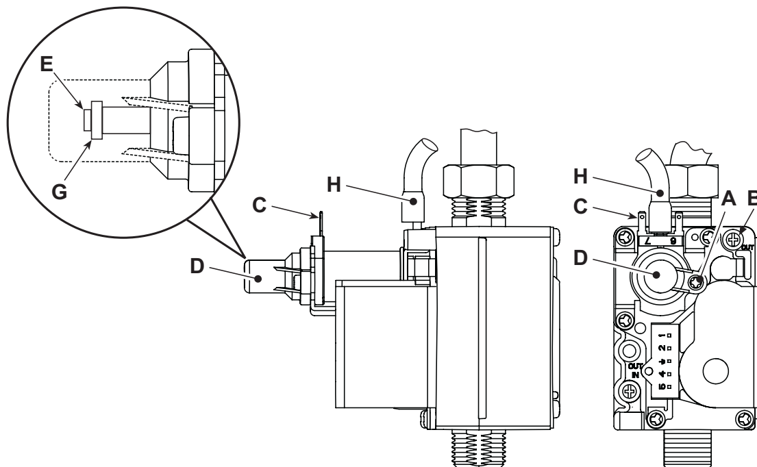
fig. 22 - Valvola gas
