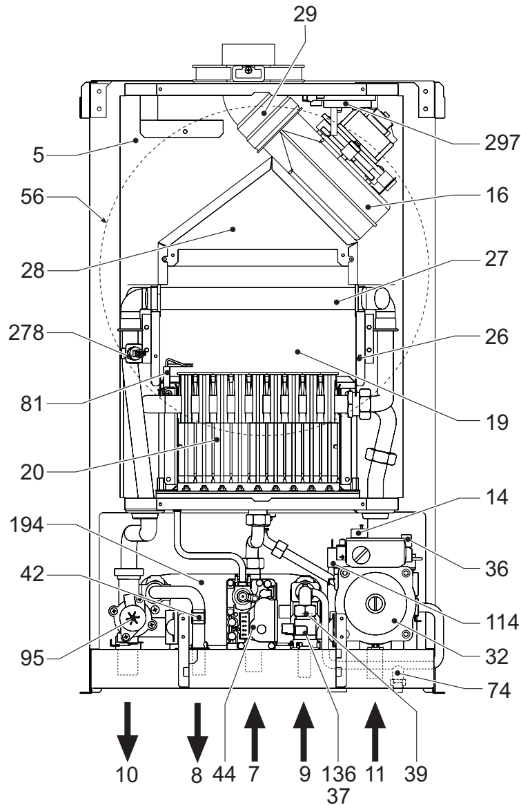
fig. 26 - General view
