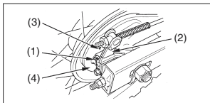
(1) Arrow (2) Brake arm (3) Reference mark (4) Brake panel
