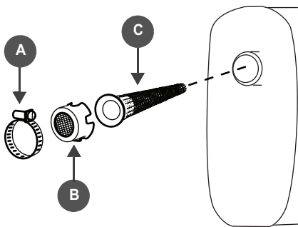
FIGURE 43: Spark Arrestor Assembly
