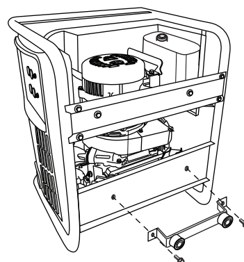
FIGURE 7: Support Leg Attached to Generator
