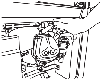
FIGURE 40: Spark Plug Cap Removal
