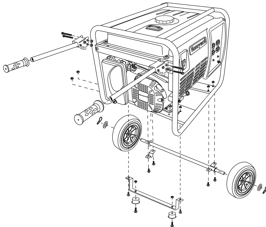
FIGURE 4: Accessory Kit Assembly
