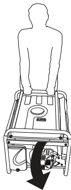
FIGURE 49: Tip Generator to Completely Drain Fuel
