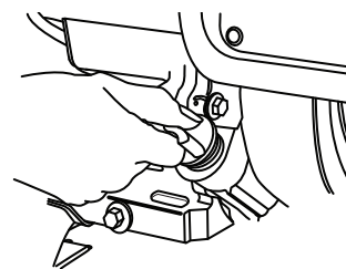
FIGURE 24: Oil Fill Dipstick Removal
