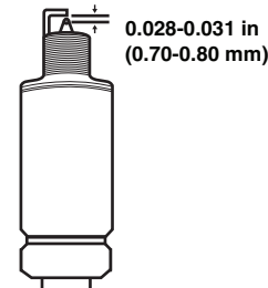
FIGURE 42: Correct Spark Plug Gap
