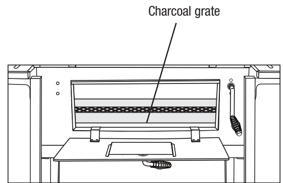
Lower Charcoal Grate Level (Smoking)
