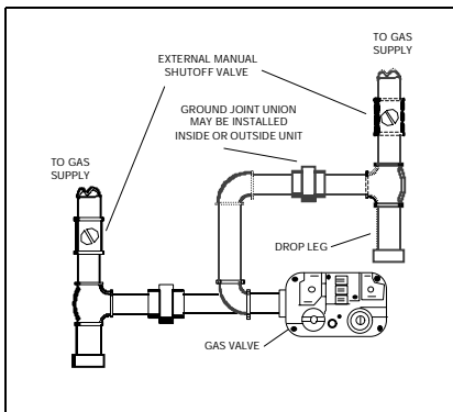
TYPICAL GAS PIPING
