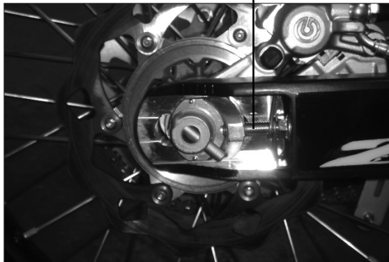
Chain tensioner
