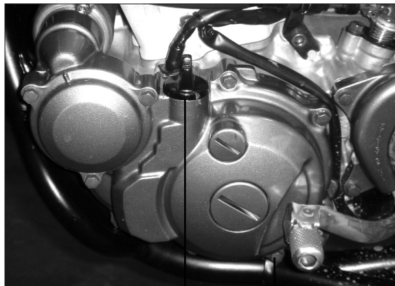
Filling cork and level hole
