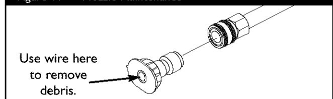
Figure 11 — Nozzle Maintenance
