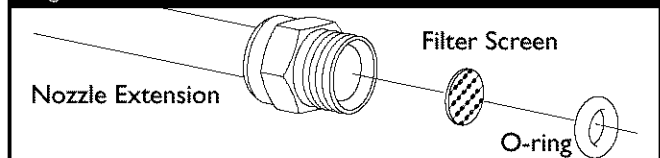
Figure 10 — Clean In-Line Filter
