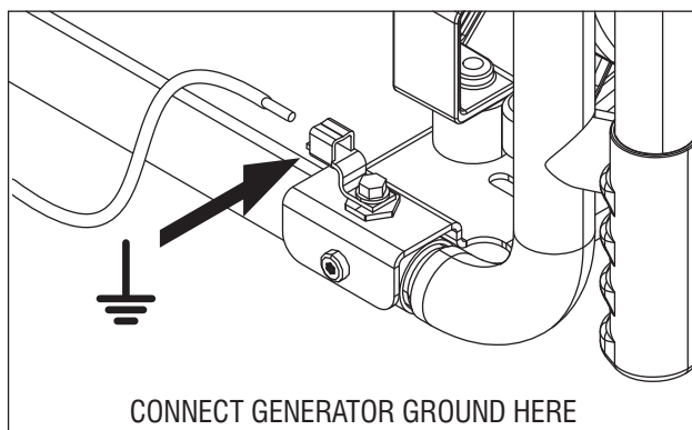
Figure 6 - Grounding the Generator
