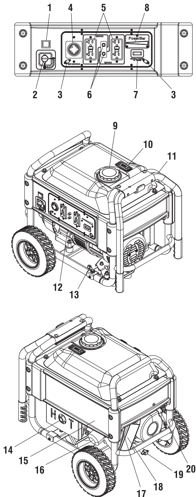
Figure 3 – Generator Locations and Controls
