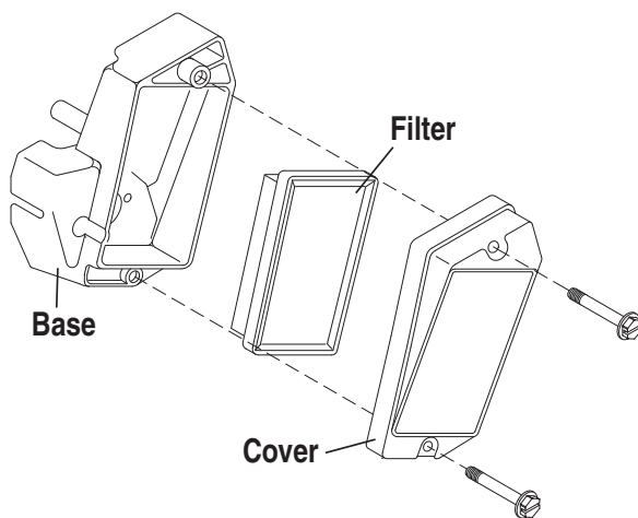
Figure 13 – Air Filter
