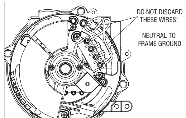
Figure 7 - Neutral to Frame Ground Wires
