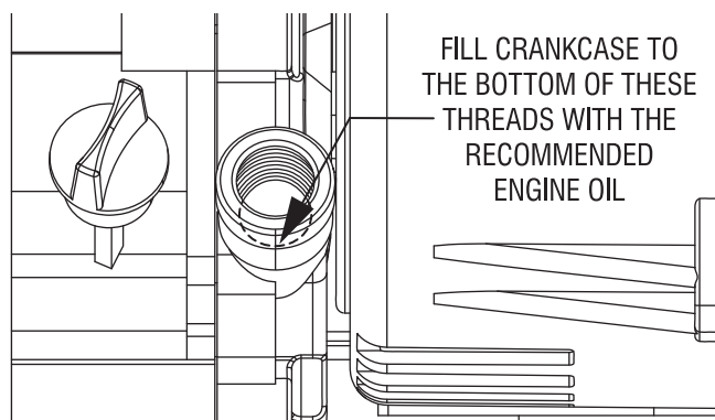
Figure 8 - Oil Level
