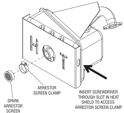
Figure 14 — Spark Arrestor Screen
