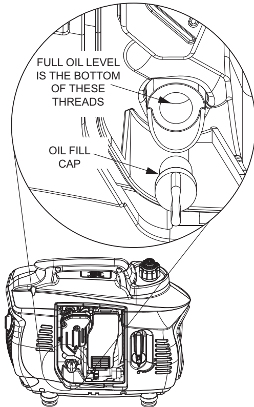
Figure 9 - Oil Fill
