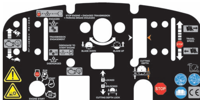
P/N 502 24 01-03 Location: Top of Cowl, FS 520, FS 524
