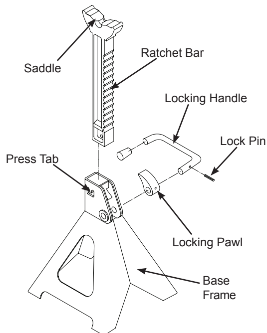
Figure 2 - Jack Stand Components
