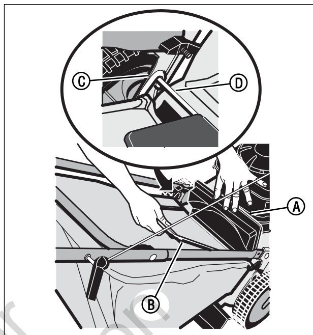
Figure 7: Mounting the grass bag
