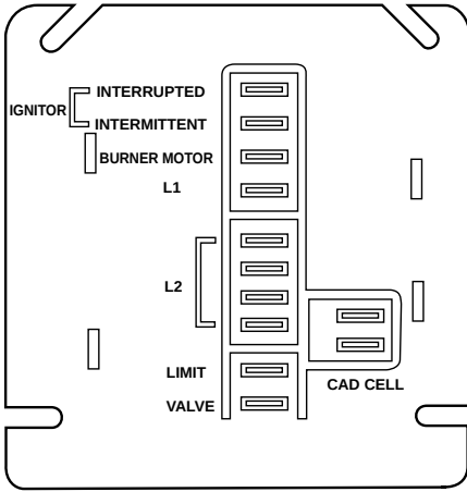
Fig. 2. Wiring terminals.
