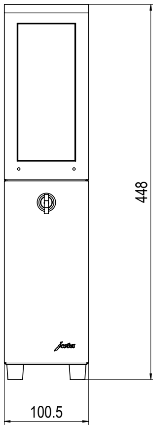
Vista frontal
