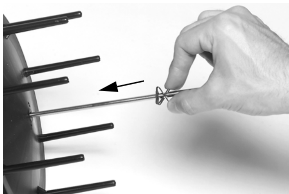
Fig. 17. Installing Spring Retainer.
