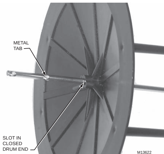
Fig. 16. Installing Closed Drum End.
