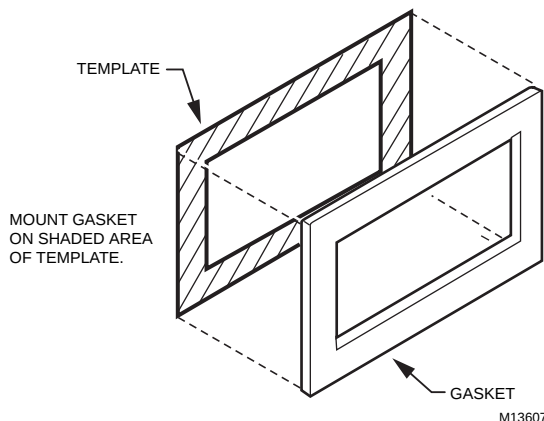
Fig. 38. Installing Gasket.
