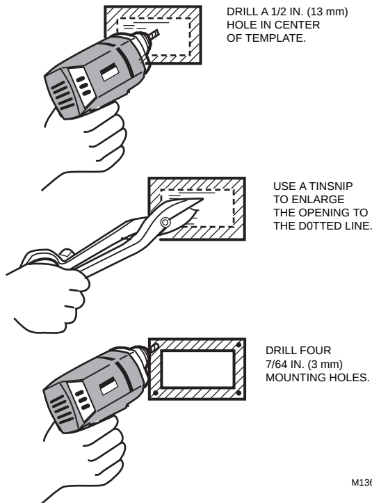
Fig. 37. Cutting Humidistat opening.
