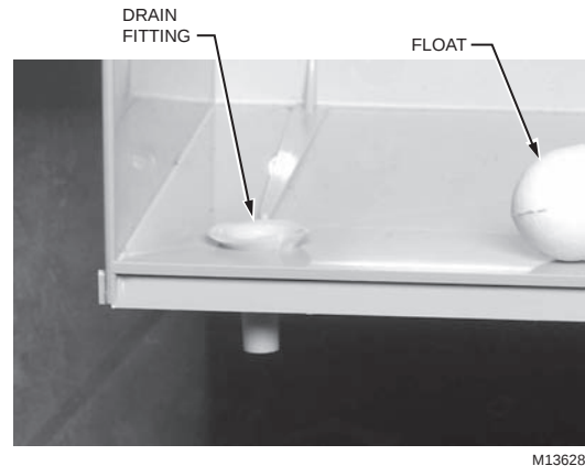
Fig. 27. Installing Drain Fitting.
