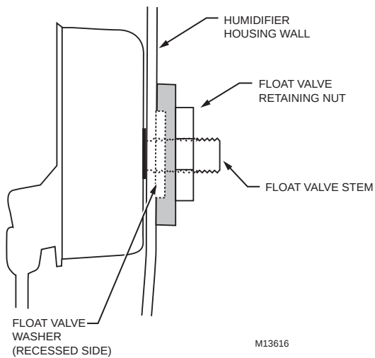
Fig. 25. Re-installing Float Valve.
