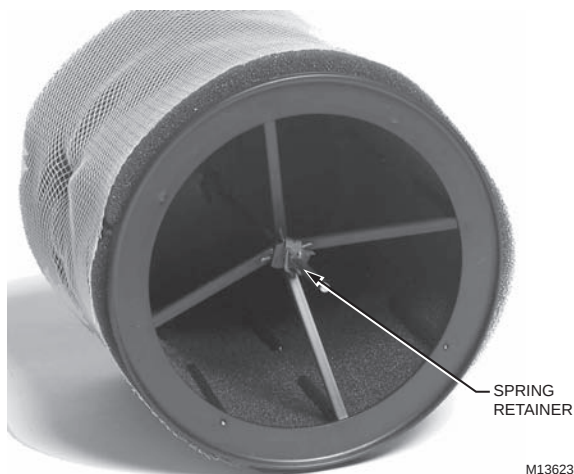
Fig. 19. Installing Open Drum End.
