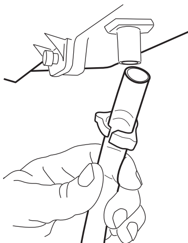
Fig. 30. Installing overflow tube.
