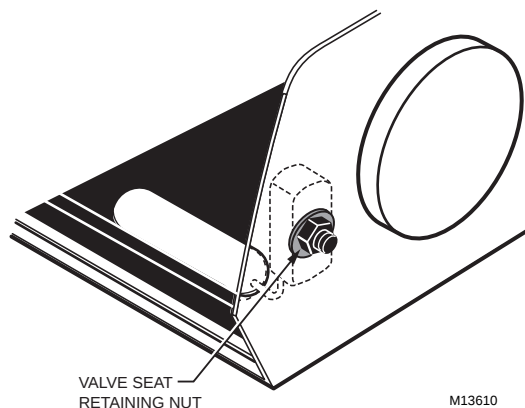
Fig. 23. Float Valve Retaining Nut.
