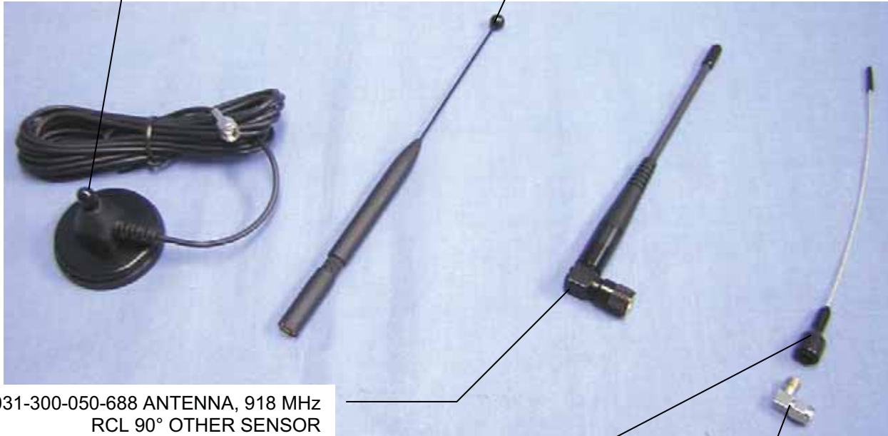
031-300-060-559 ANTENNA ASSY, 918 MHz WHIP FOR LOAD CELL FOR LOAD SENSOR
