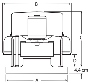
Figure 1 — Dimensions
