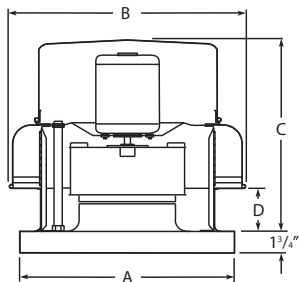
Figure 1 — Dimensions
