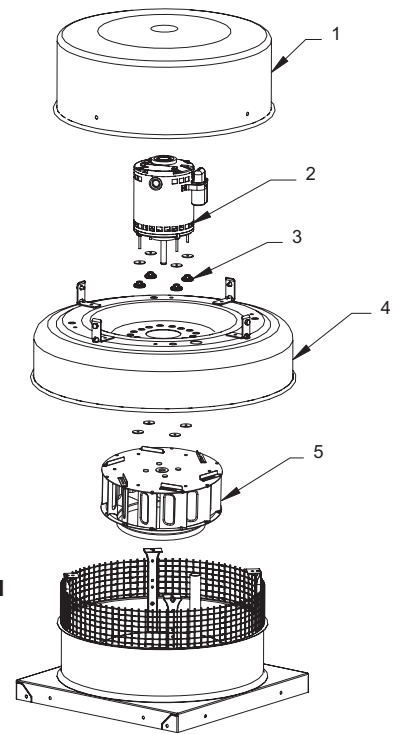
Figure 5 – Repair Parts Illustration for Centrifugal Direct-Drive Downblast Exhaust Ventilators
