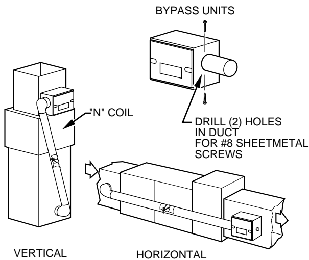
→ Fig. 14—Installation of HUMBWTR2019-A-- Water Saver Humidifier
