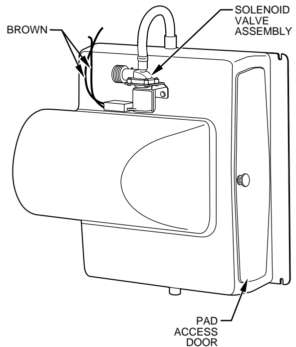
→ Fig. 13—Mounting Solenoid Valve on HUMBBSP2017-A-- Humidifier
