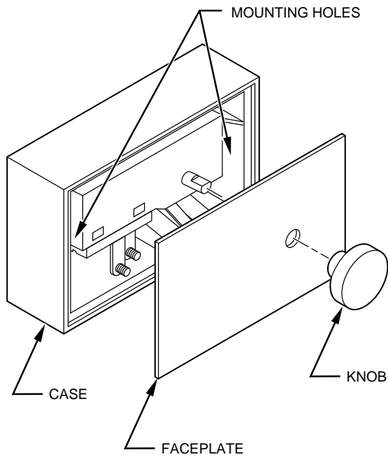
Fig. 18—Knob and Faceplate Removal
