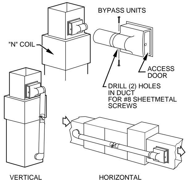
→ Fig. 12—Installation of HUMBBSP2017-A-- Bypass-Type Humidifier
