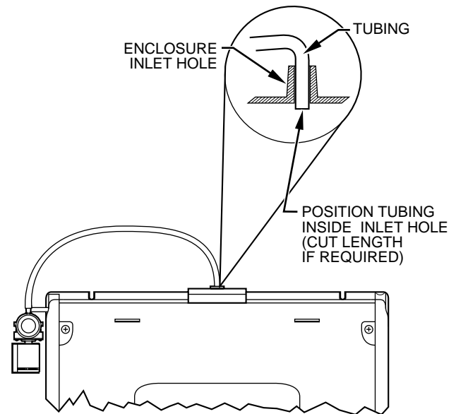
Fig. 11—Alternate Mounting of Solenoid Valve on HUMBSFP1016-A-- Humidifier
