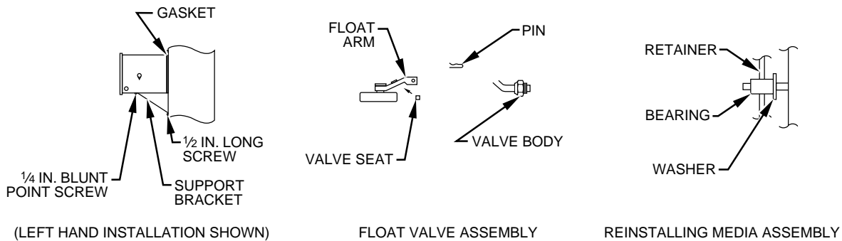
→ Fig. 15—Valve and Media Assembly for HUMBBWTR2019-A--
