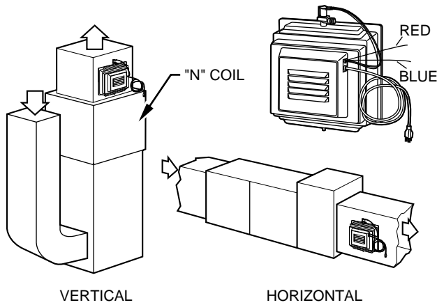
→ Fig. 5—Installation of HUMBLFP1025-A-- Fan-Type Humidifier
