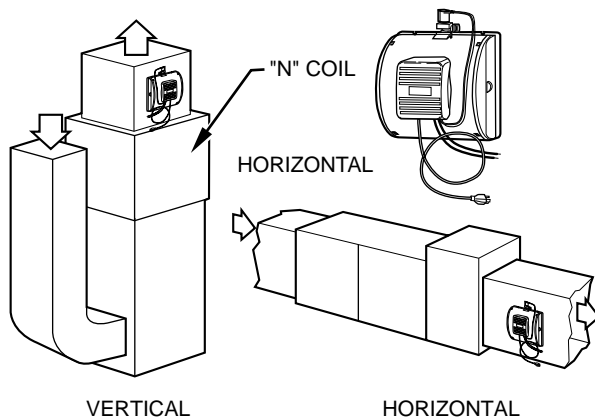
Fig. 7—Installation of HUMBBSFP1016-A-- Fan-Type Humidifier
