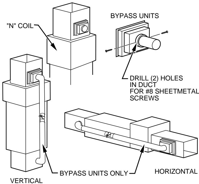
→ Fig. 1—Installation of HUMBBLBP2018-A-- Bypass-Type Humidifier
