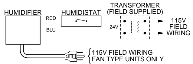
Fig. 6—Installation of Humidistat on Fan-Type Humidifier
