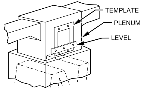
Fig. 2—Preparing Plenum Opening
