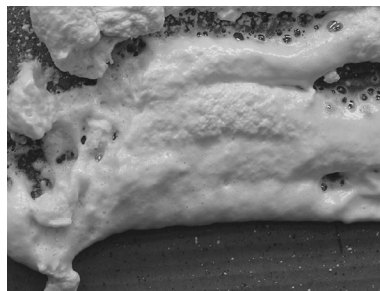
B-rich Foam
