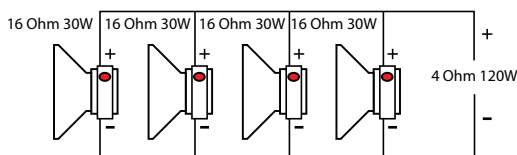
PARALLEL CONNECTION
