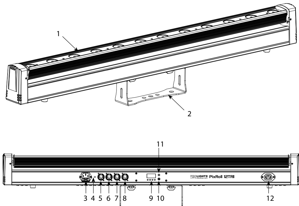
Rear panel
