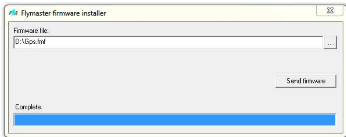
Figura 37 – Firmware Installer
