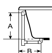
DRAIN/OVERFLOW
