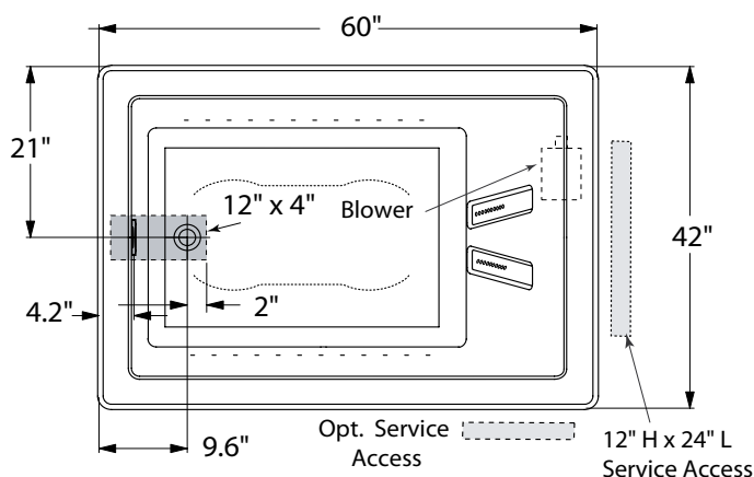
Product Shown: Elara™ 6042 Pure Air® Left Hand Model: GA70
