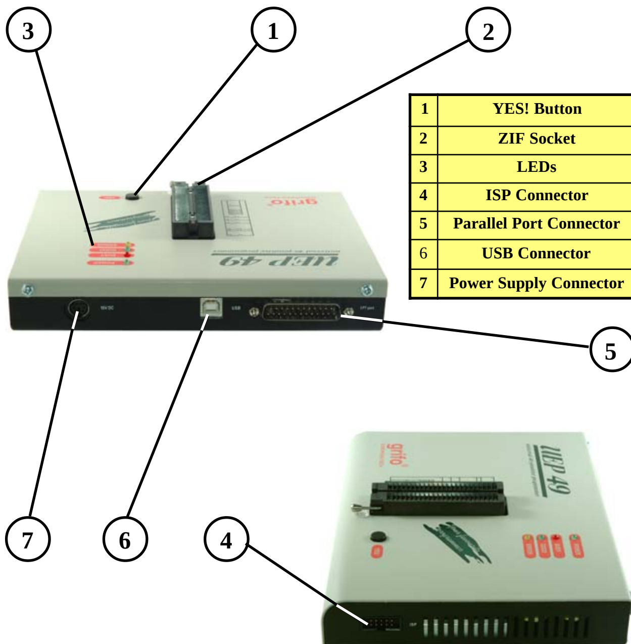
FIGURE 9: CONNECTORS, LEDs, ETC. LOCATION
