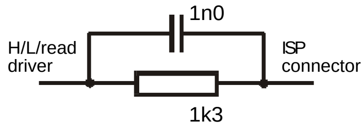
FIGURE 4: ISP DRIVER OF UEP 49
