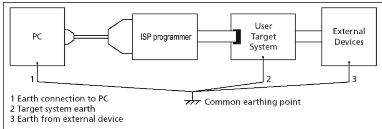
FIGURE 3: ISP CONNECTION EXAMPLE
