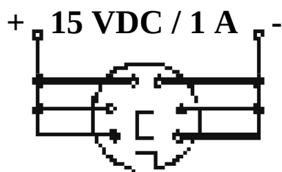
FIGURE 10: POWER SUPPLY CONNECTOR
