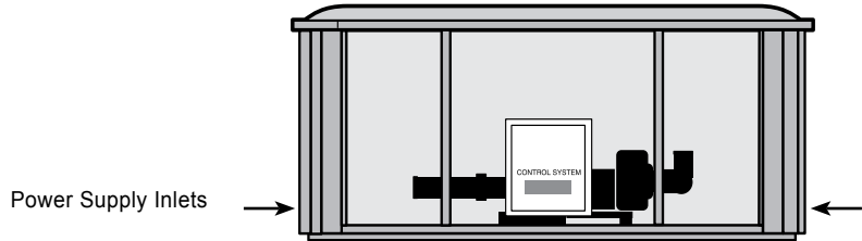
Figure 6 The Spa Equipment Compartment
