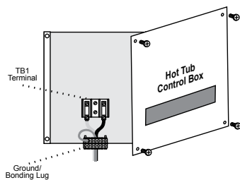
Figure 4: Control Box
