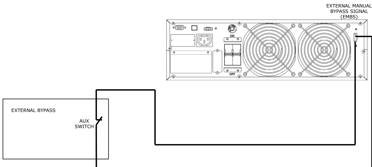
Figure 7 - Connection EXTERNAL BYPASS to EMBS terminals
