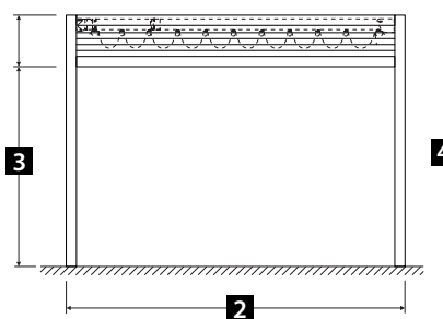
PT100 IN PIANO
