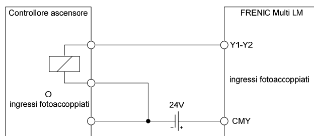
Figura 4.10 Collegamento mediante logica PNP (source)
