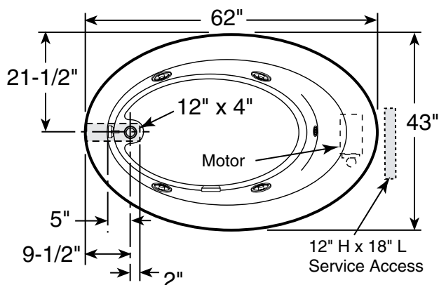
Product Shown: Riva™ 5 Whirlpool Bath Left Hand Shown Model: 9330
