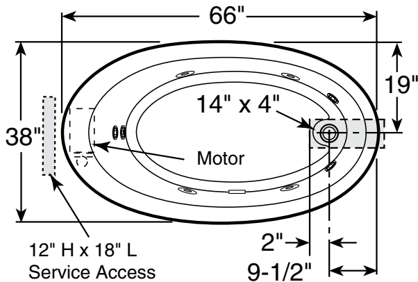
Product Shown: Riva® 5.5 Whirlpool Plus Right Hand Shown Model: FX05
