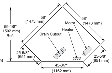
CAPELLA™ 60 PLUS, Right Hand CUTOUT
