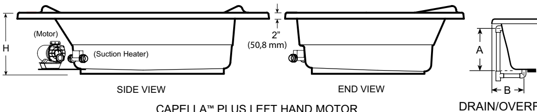
CAPELLA™ PLUS LEFT HAND MOTOR
