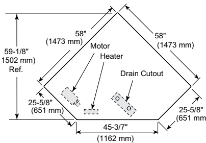
CAPELLA™ 60 PLUS, Left Hand CUTOUT
